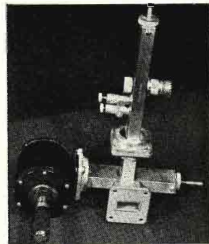
Figure 4 High frequency discriminator.
