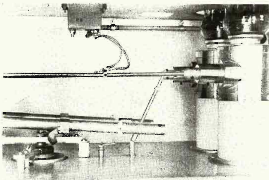
Figure 2 Position of the plate tank and output circuit of the power amplifier
