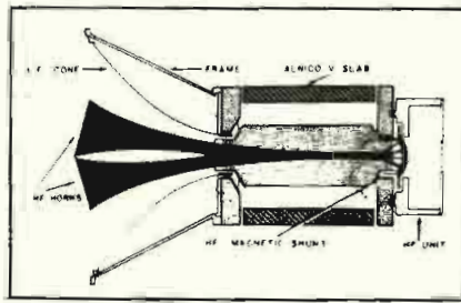
Figure 5 Coaxial unit design.
