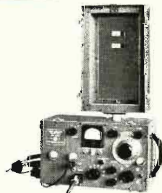
FEDERAL'S Field Intensity Meter accurately measures signal intensity of AM broadcasting stations whether in the standard band of 530-1600 Kc—200 to 400 Kc—1600 to 3600 Kc—or 3600 to 7000 Kc. This 29-lb. unit is portable.
