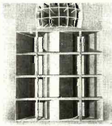
Figure 1 An 80-watt separate two-way theatre system.
