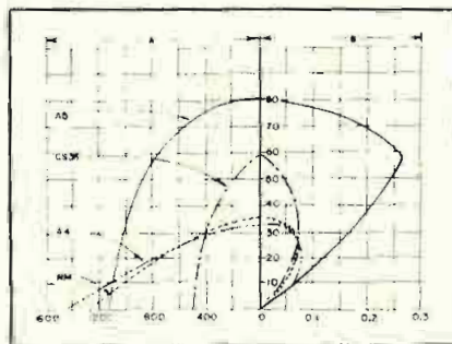
Figure 7 Demagnetization and external energy curves for permanent magnet steels: A , ampere turns per square inch (H) and B , energy in air gap per cubic inch of iron (joules) for Alnico 5 (A5), Alnico 4 (A4), cobalt steel 36% (CS-36) and Nipermag (NP).
