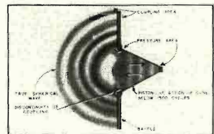
Figure 10 Acoustic action of a cone radiator below 1500 cycles.
