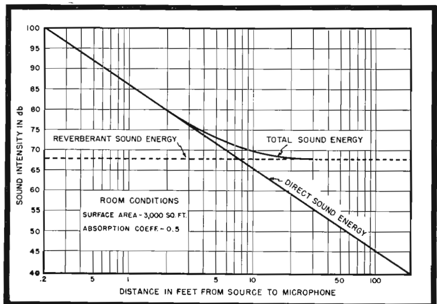
Figure 1 Approximate relationship between direct and reverberant sound.
